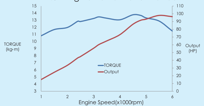
1.5L Engine Power Performance
